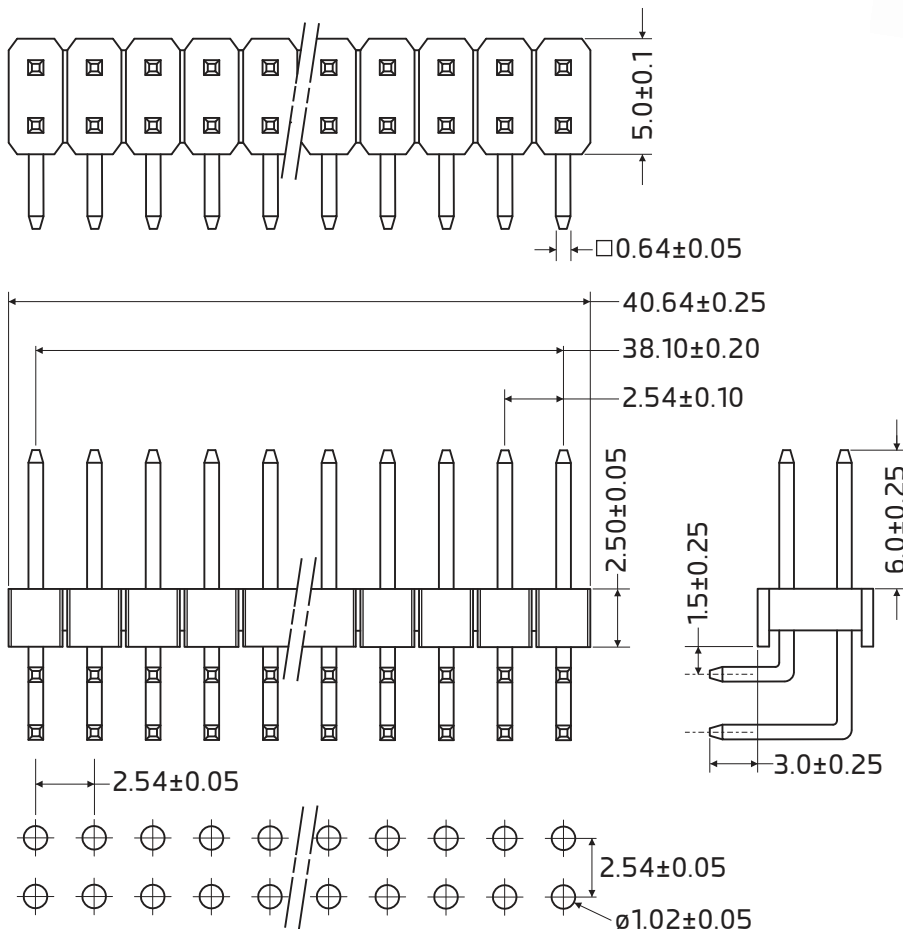
Recommended Board Hole Layout
