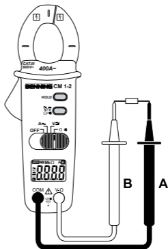
BENNING CM 1-2
