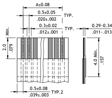
Accommodated FFC/FPC
