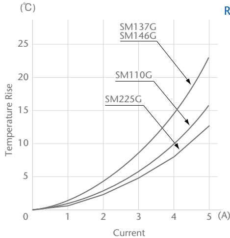
Temperature Rise
